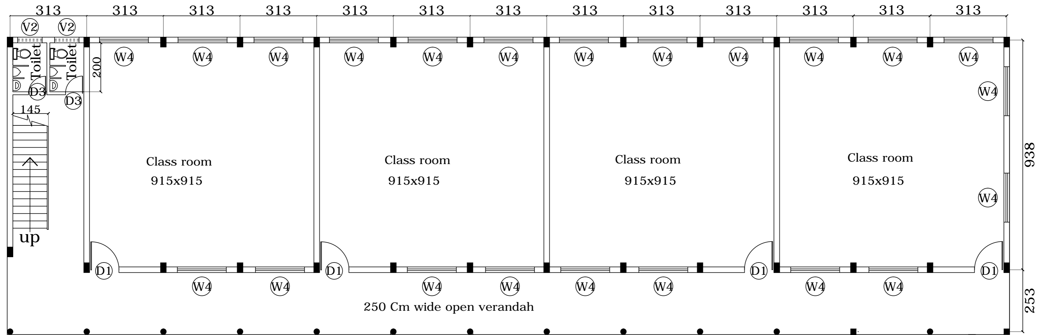
GROUND FLOOR PLAN PLINTH AREA- 497 SQM
