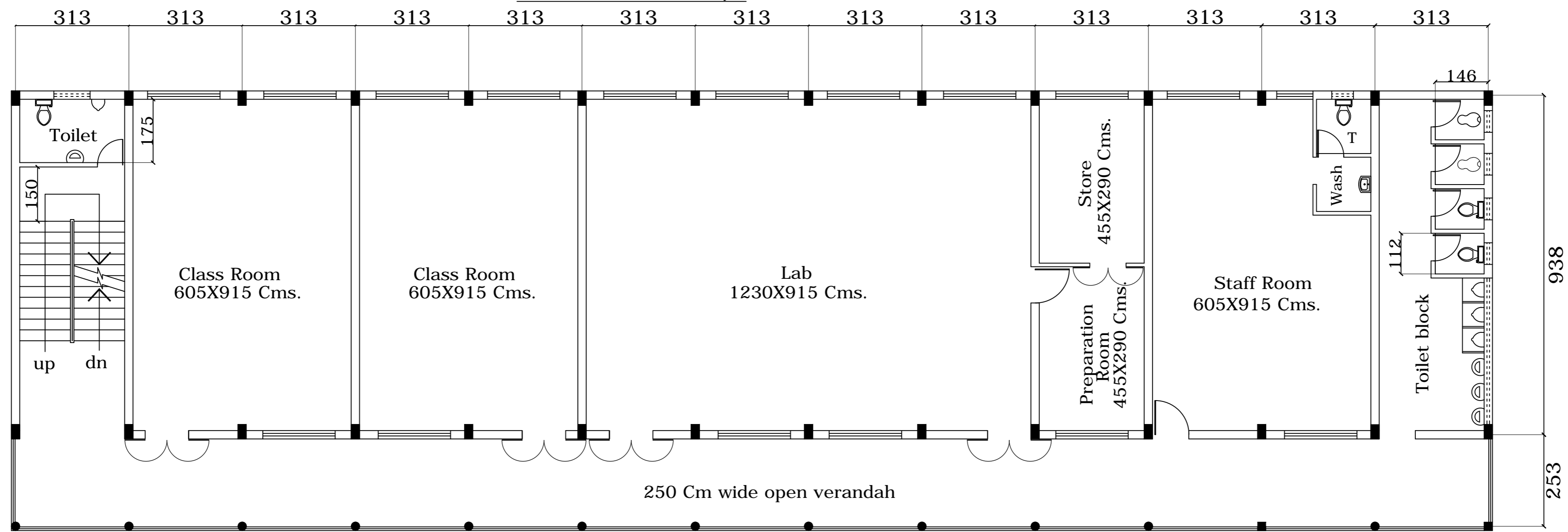
THIRD FLOOR PLAN
