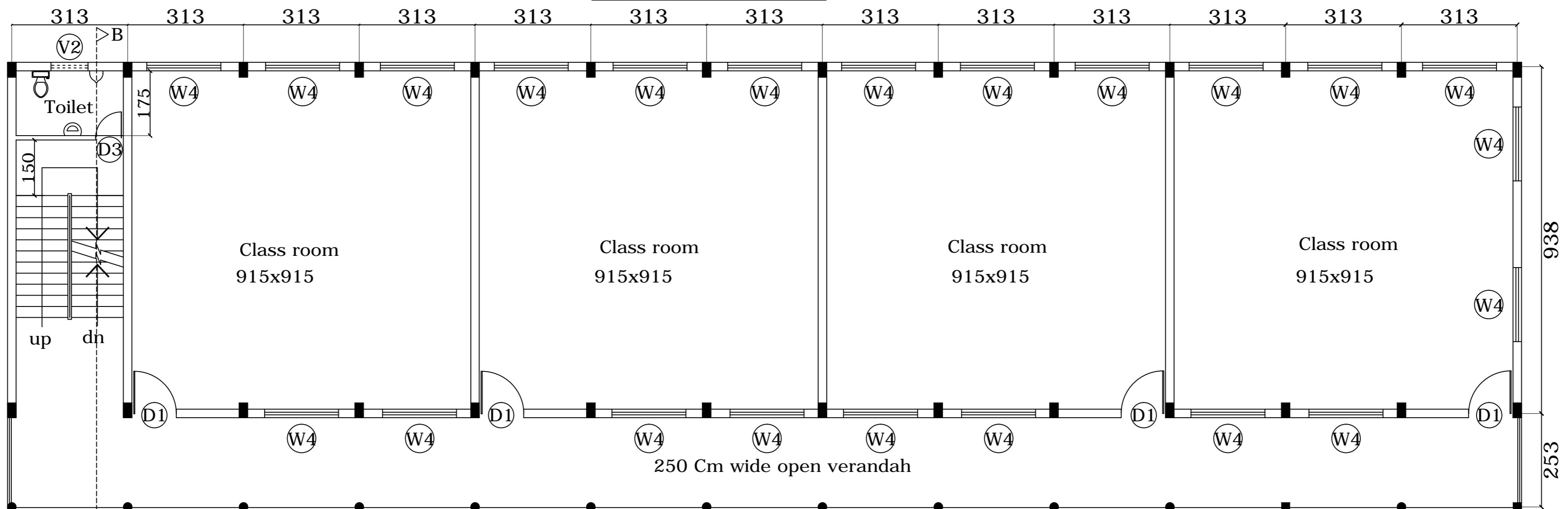
FIRST FLOOR PLAN PLINTH AREA- 497 SQM
